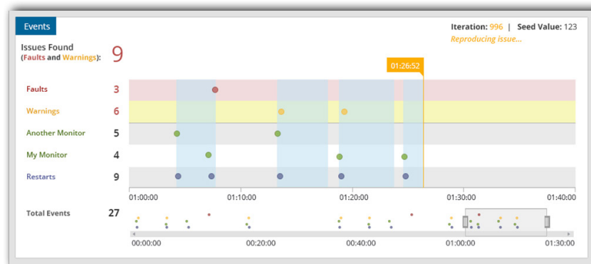
Real-time instantaneous fuzzing results.
